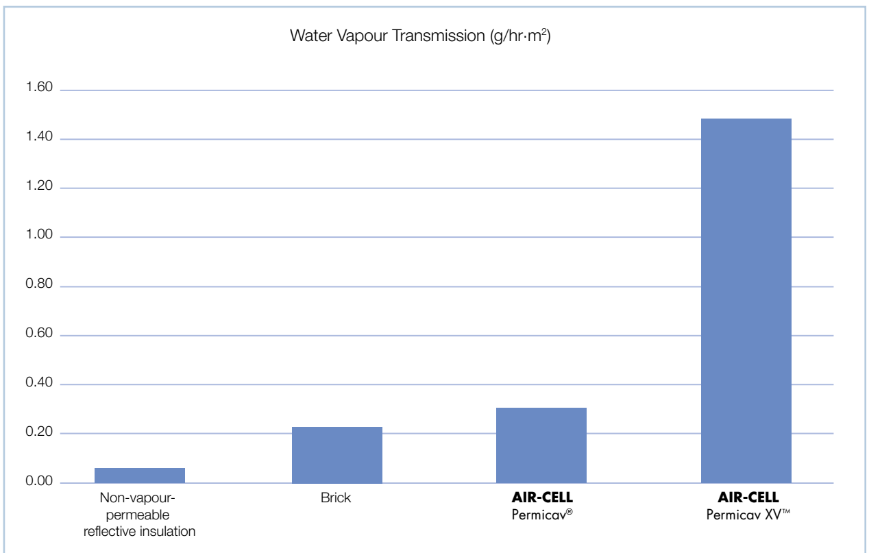
Figure 6 Water vapour transmission comparison.
