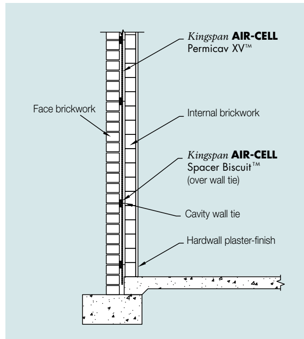
Figure 2 Side elevation of Kingspan AIR-CELL Permicanv XV™ in double brick cavity wall
