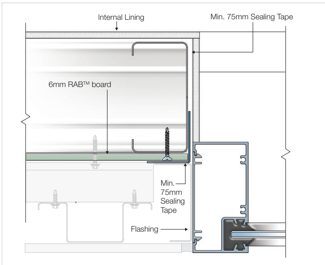
FIGURE 17 FLUSH WINDOW JAMB
