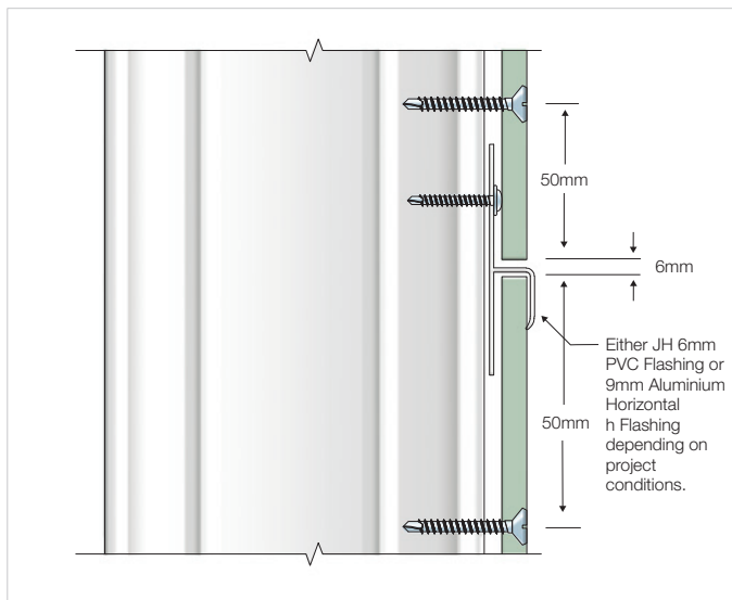
FIGURE 12 HORIZONTAL JOINT
