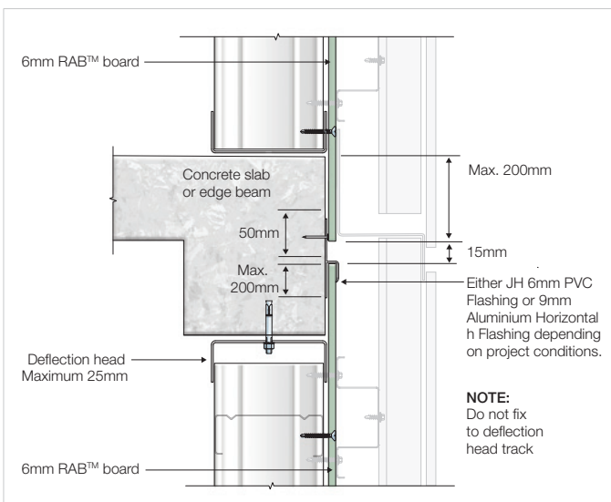
FIGURE 6 HORIZONTAL SLAB JUNCTION (CONTINUOUS)
