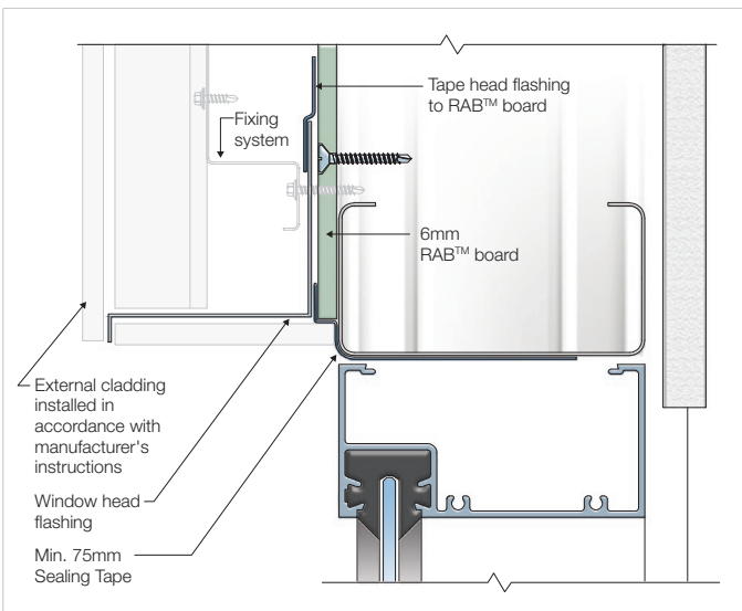
FIGURE 23 RECESSED WINDOW HEAD
