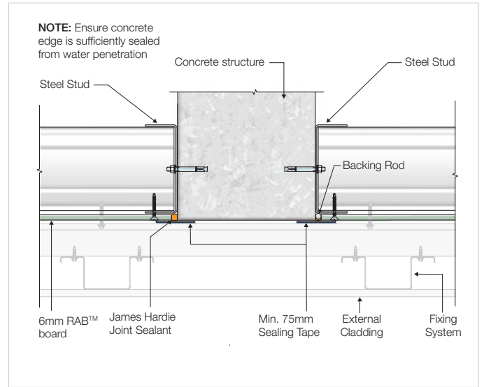
FIGURE 9 VERTICAL COLUMN JUNCTION (BUTTED)
