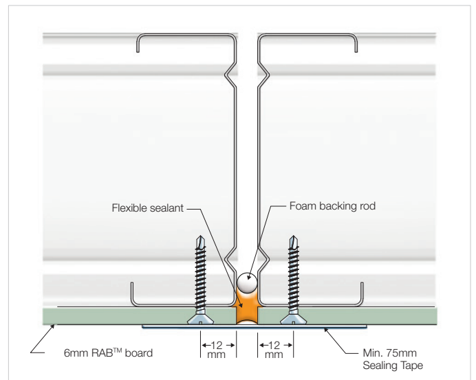
FIGURE 13 VERTICAL CONTROL JOINT
