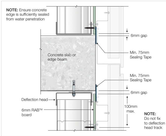
FIGURE 8 HORIZONTAL SLAB JUNCTION (BUTTED)
