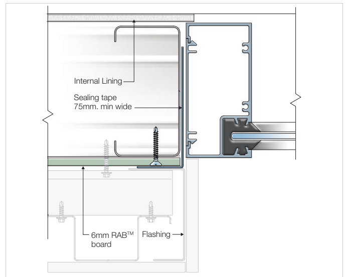
FIGURE 22 RECESSED WINDOW JAMB
