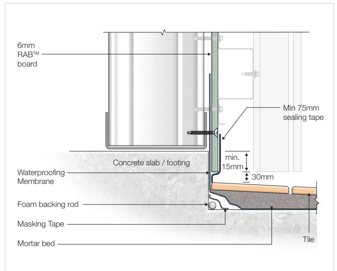
FIGURE 5 BASE DETAIL BALCONY
