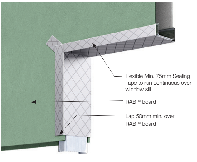
FIGURE 21 WINDOW CORNER TAPING DETAIL
