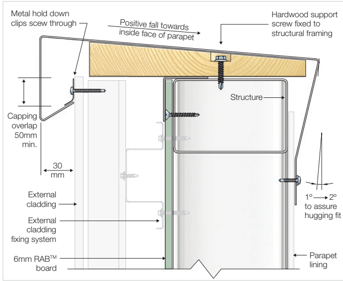
FIGURE 25 PARAPET DETAIL
