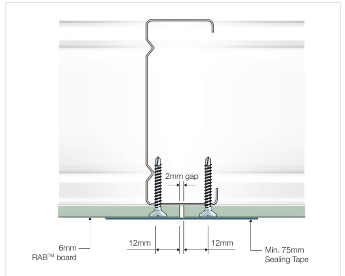
FIGURE 11 VERTICAL JOINT
