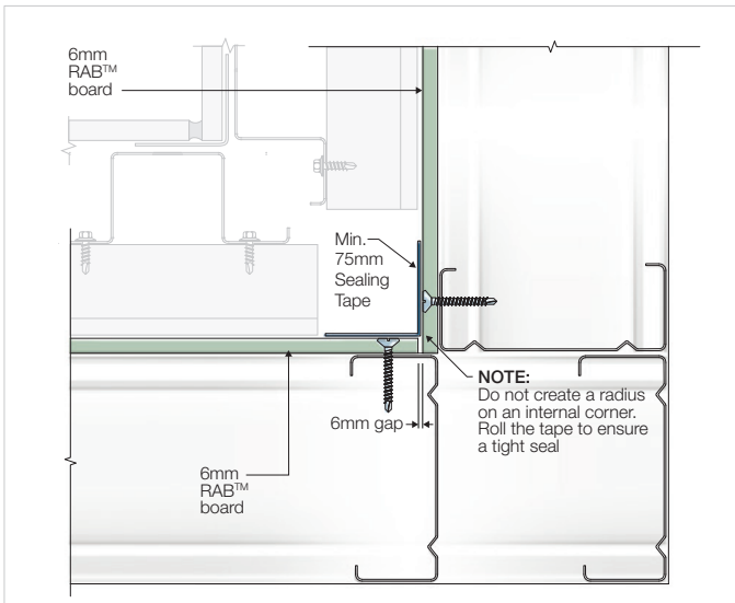
FIGURE 16 INTERNAL CORNER
