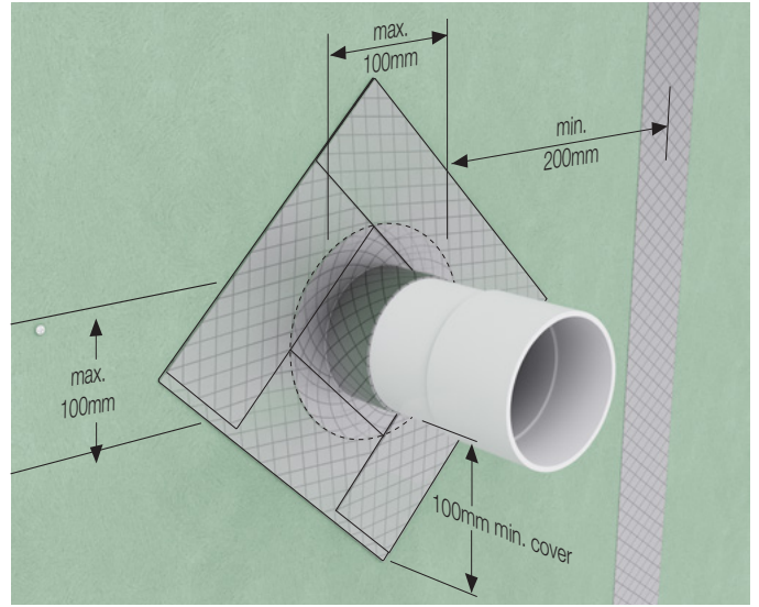
FIGURE 26 PIPE AND OTHER PENETRATIONS
