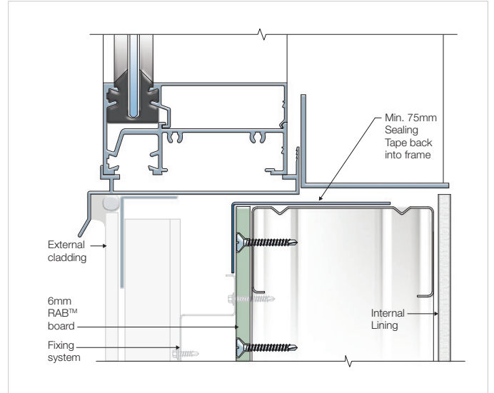
FIGURE 20 FLUSH WINDOW SILL
