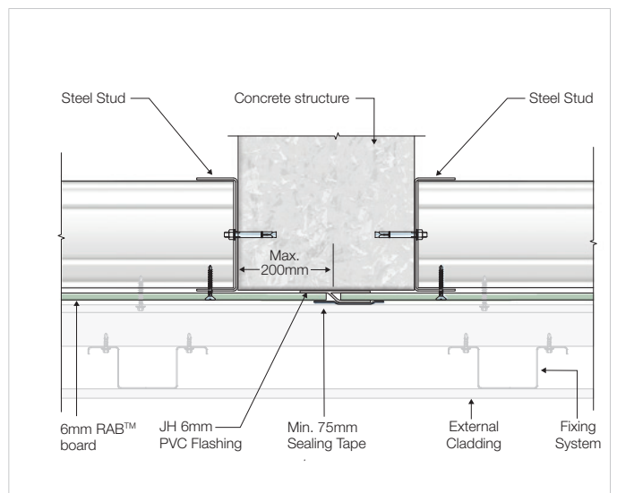
FIGURE 7 VERTICAL COLUMN JUNCTION (CONTINUOUS)
