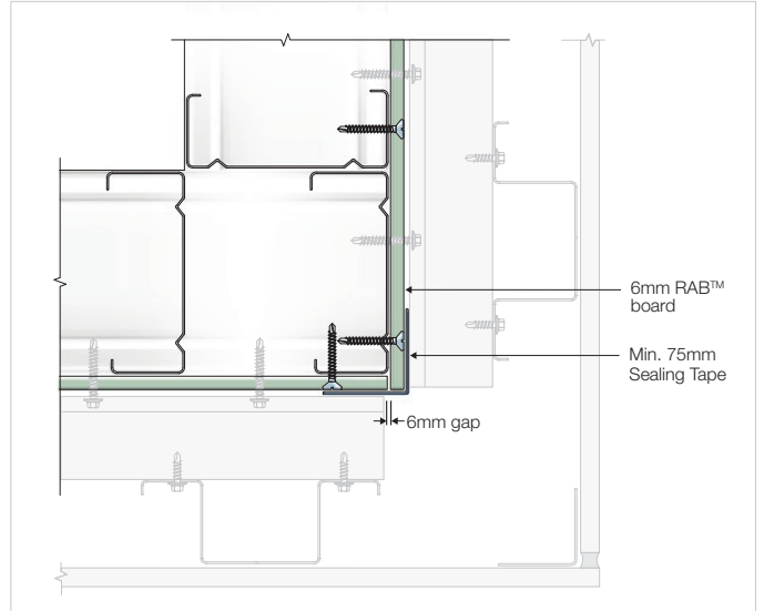
FIGURE 15 EXTERNAL CORNER
