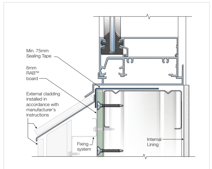
FIGURE 24 RECESSED WINDOW SILL
