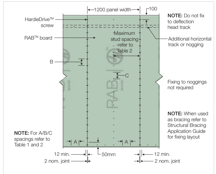
FIGURE 3 FIXING LAYOUT FOR STRUCTURAL BRACING
