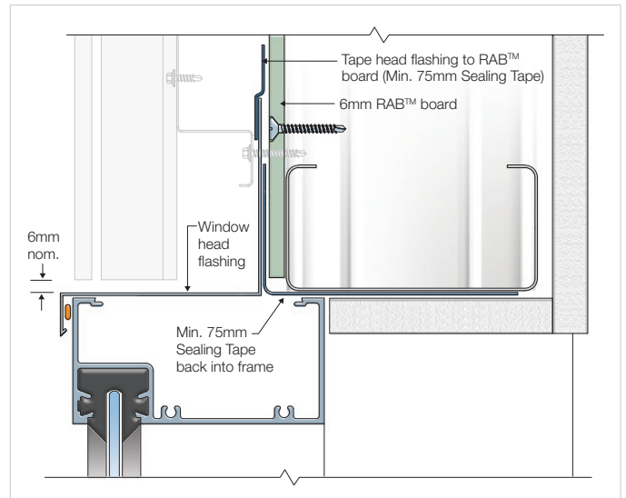
FIGURE 18 FLUSH WINDOW HEAD
