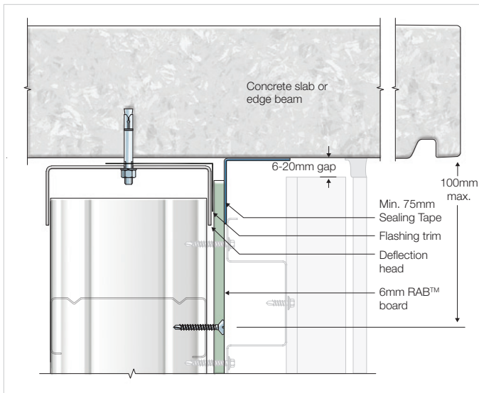
FIGURE 10 UNDER SLAB JUNCTION
