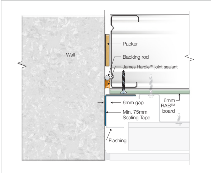
FIGURE 14 ABUTMENT TO MASONRY WALL FOR BALCONY INFILL
