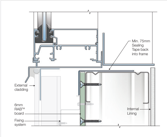
FIGURE 19 FLUSH WINDOW SILL
