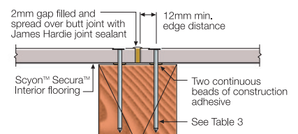
FIGURE 6 BUTT JOINING OPTIONS
