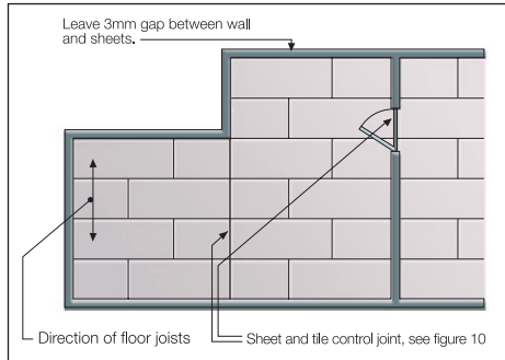
FIGURE 9 L-SHAPED ROOM
