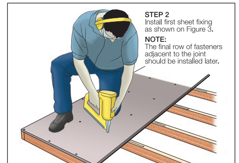
FIGURE 4 FIXING 1ST PANEL
