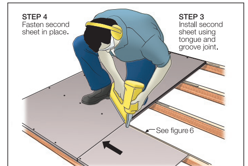
FIGURE 5 FIXING 2ND PANEL
