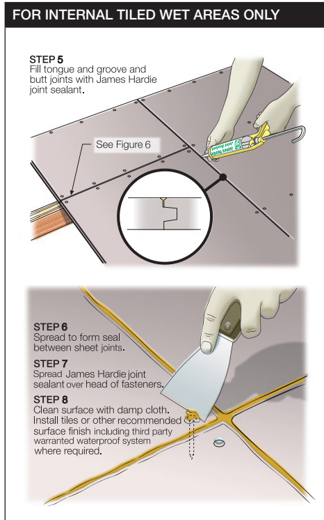
FIGURE 8 SEALING FASTENER JOINTS - WET AREAS NOTE: Avoid excessive foot traffic on the floor for at least 24-48 hours to allow sealant to set and dry out. Protect the surface of the sheets from damage until final finish is applied.
