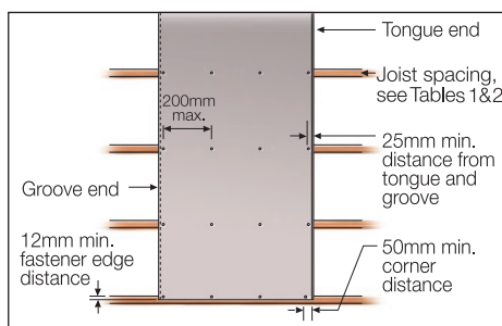
FIGURE 3 FASTENER LAYOUT
