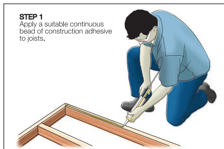
FIGURE 2 CONSTRUCTION ADHESIVE
