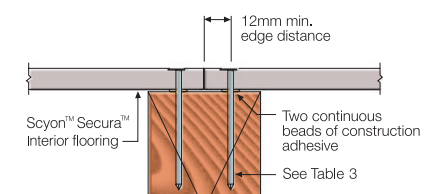
FIGURE 5 FIXING 2ND PANEL
