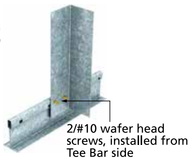
WAH/SA12 secured to tee web
