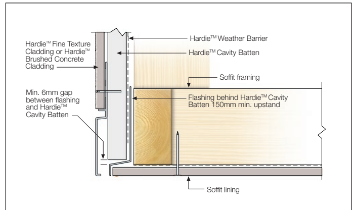
FIGURE 28 FACADE/SOFFIT JUNCTION
